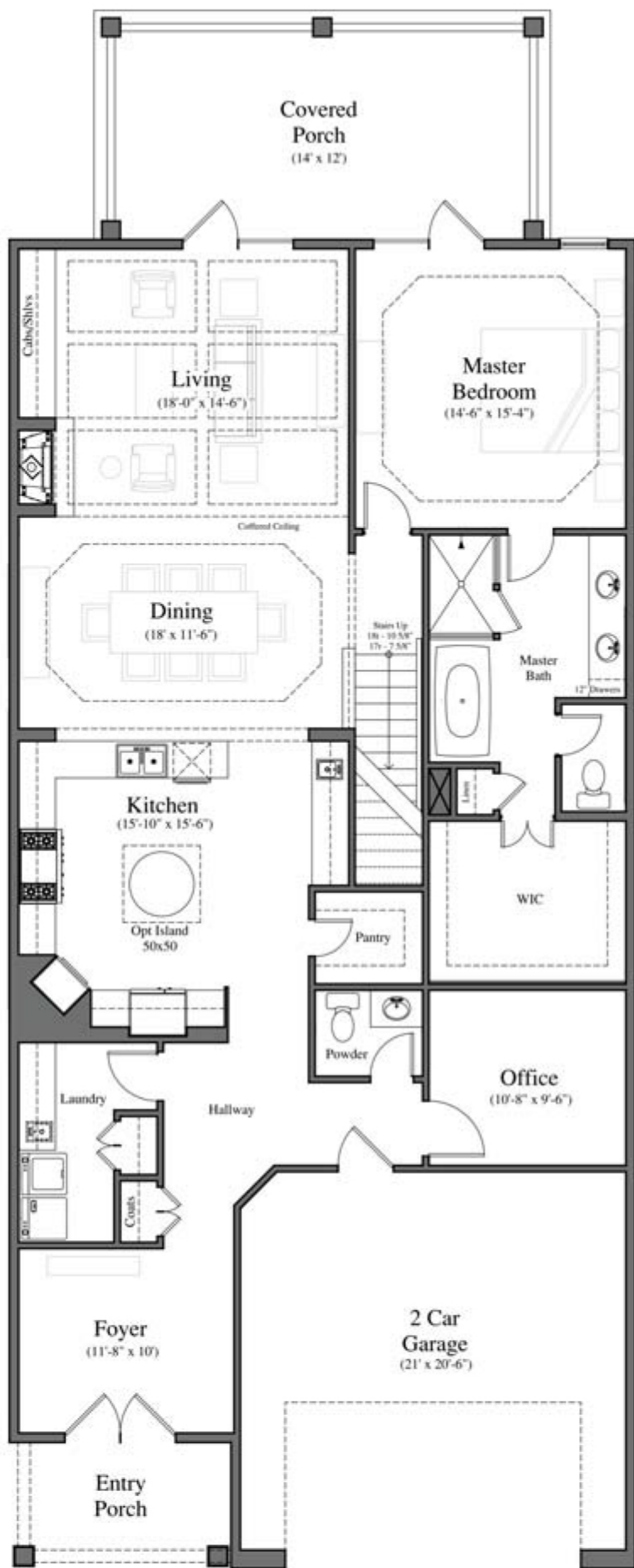
Main Level
